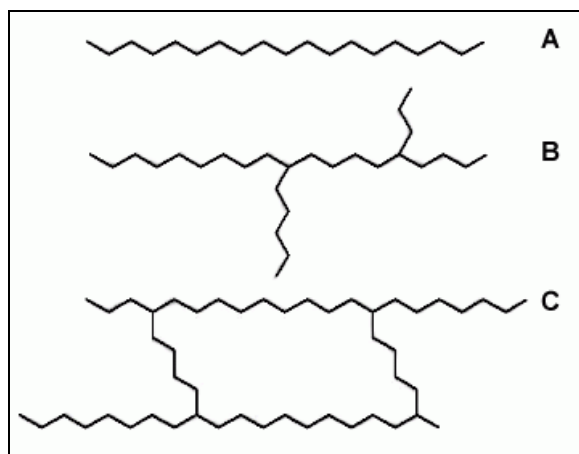
Figure 1.1: Basic structures of polymers
