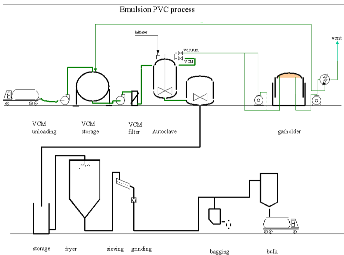
Figure 5.2: Flow diagram of an E-PVC process
