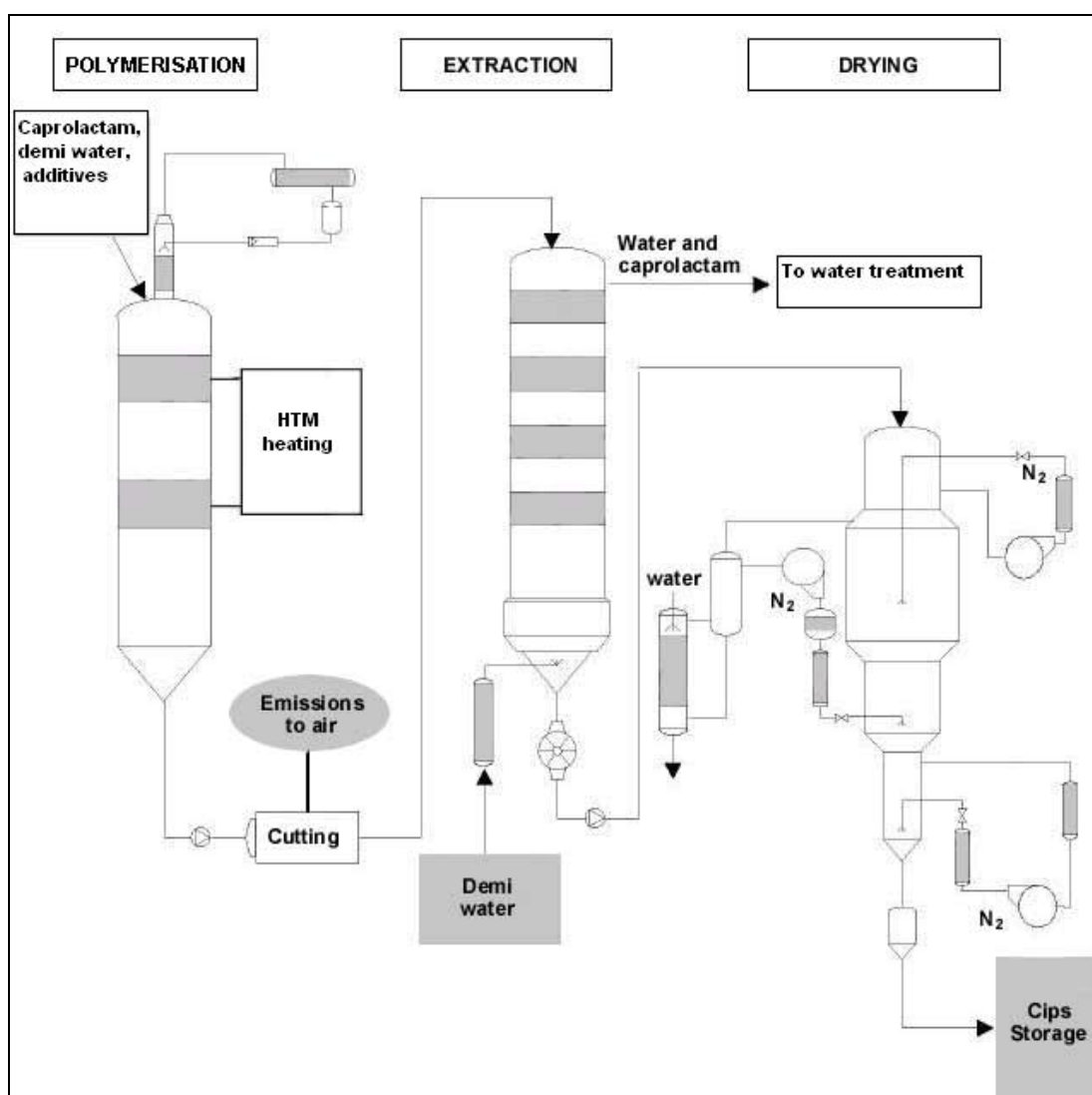
Figure 9.4: Flow diagram of the continuous PA 6 process
