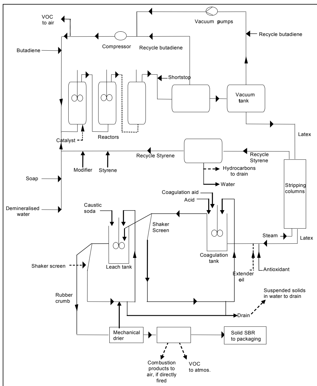
Figure 7.3: Flow diagram of the ESBR production process
