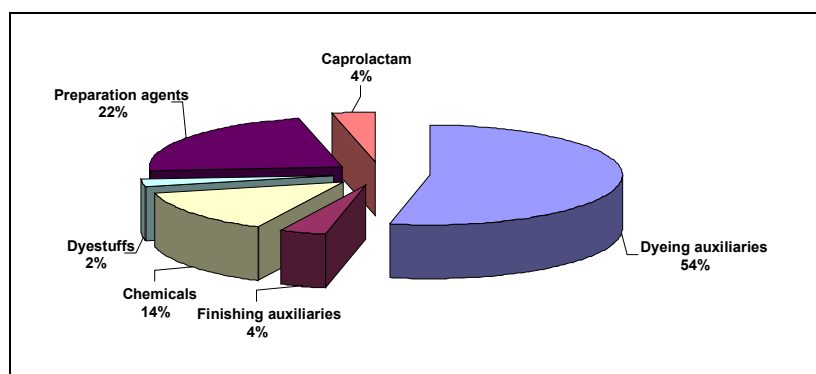
Figure 3.7: Example of composition of the COD load for a mill finishing knitted fabric consisting mainly of polyamide [179, UBA, 2001]
