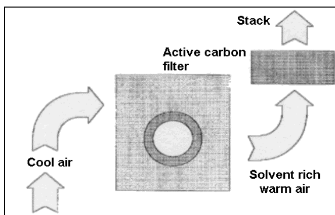
Figure 2.40: Solvent washing: representation of the air circuit in an open-loop washing machine [66, CRIT, 1999] revised by [318, Sperotto Rimar, 2002]
