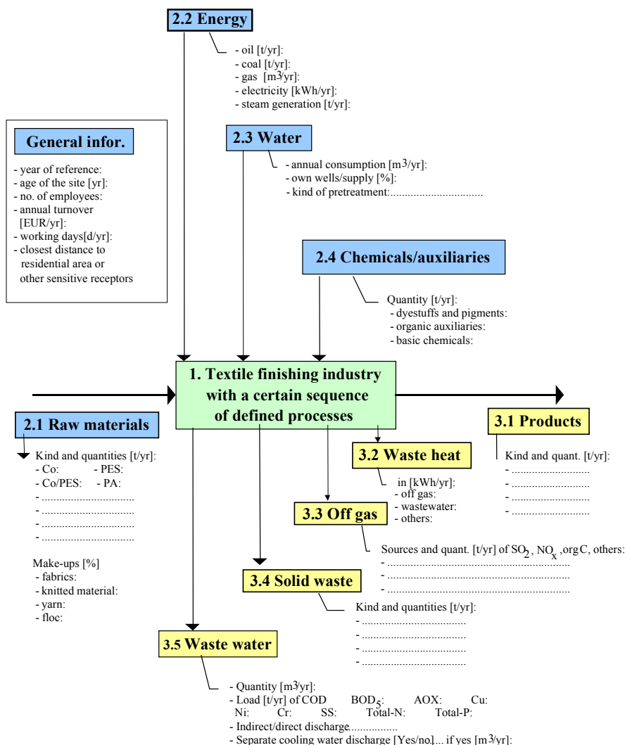
Figure 4.1: Scheme for annual input/output overview at site level [179, UBA, 2001]
