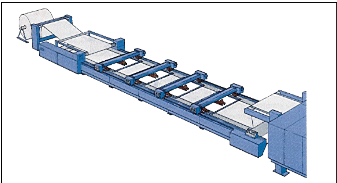
Figure 2.19: Representation of "Mechanised screen printing machine with stationary screens mounted in a frame" [69, Corbani, 1994]
