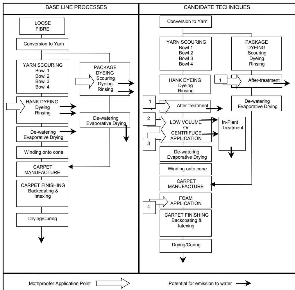
Figure 4.31: Process map for mothproofing yarn dyed production [32, ENco, 2001]
