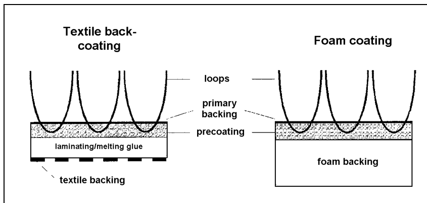
Figure 2.6: Cross-section of a tufted carpet [63, GuT/ ECA, 2000]
