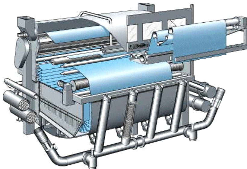
Figure 4.23: Supraflor Carpet Winch [171, GuT, 2001]
